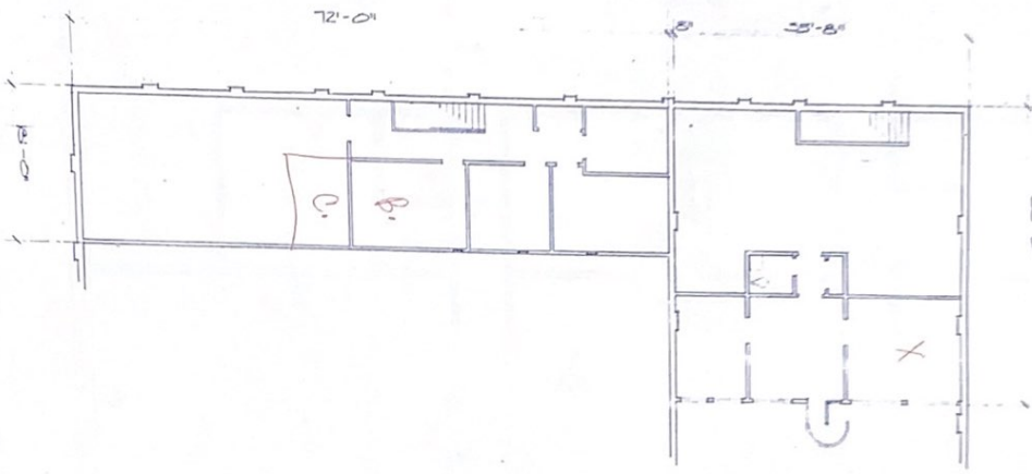
SECOND FLOOR PLAN - SHOPS A+B 5"
